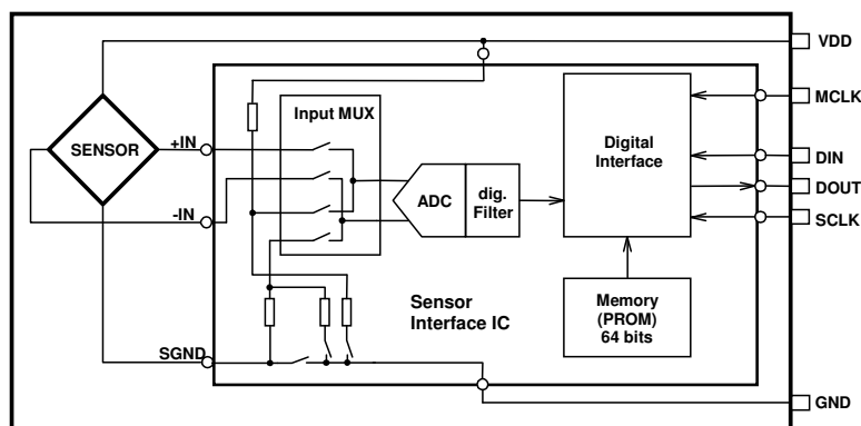
Fig. 1: Block diagram MS5535-30C
