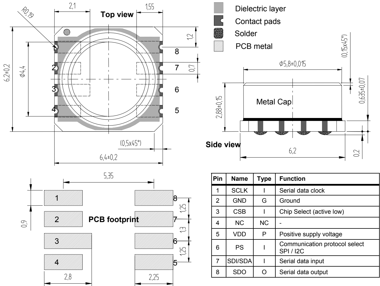
Figure 18: MS5803-05BA package outlines, recommended PCB footprint, pin configuration and description
