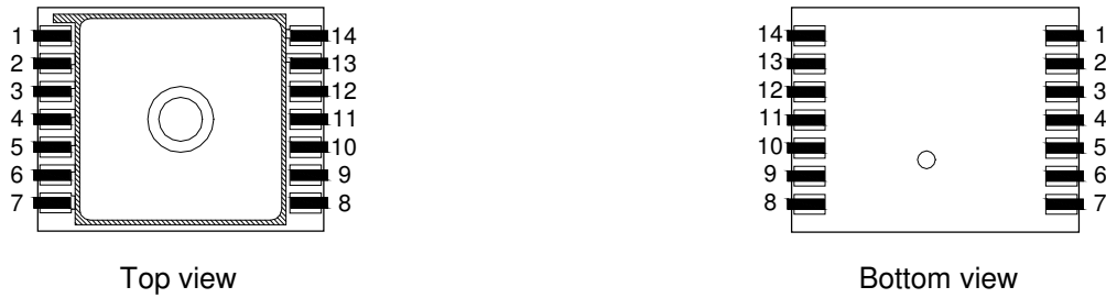
Fig. 2: Pin configuration of MS5536-PJU, MS5536-NJU
