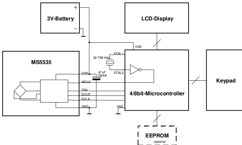
Figure 7: Demonstration of MS5535A (RoHS) in a diving computer.
