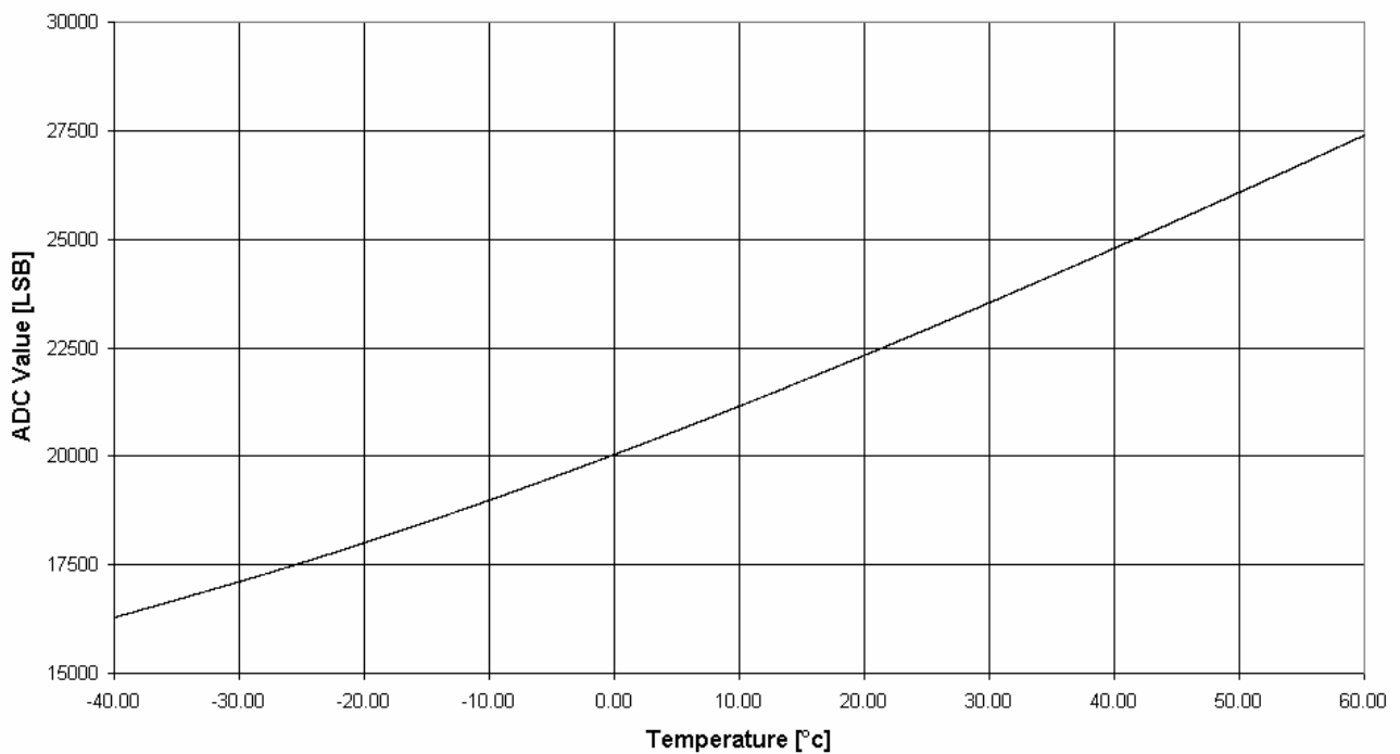
ADC-Value D2 vs Temperature
