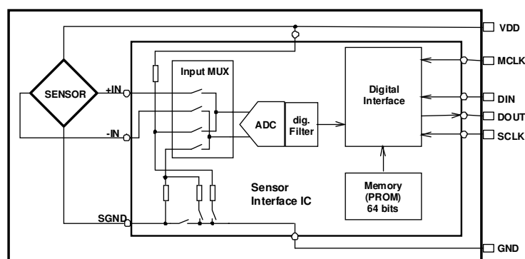
Fig. 1: Block diagram 5535A (RoHS).
