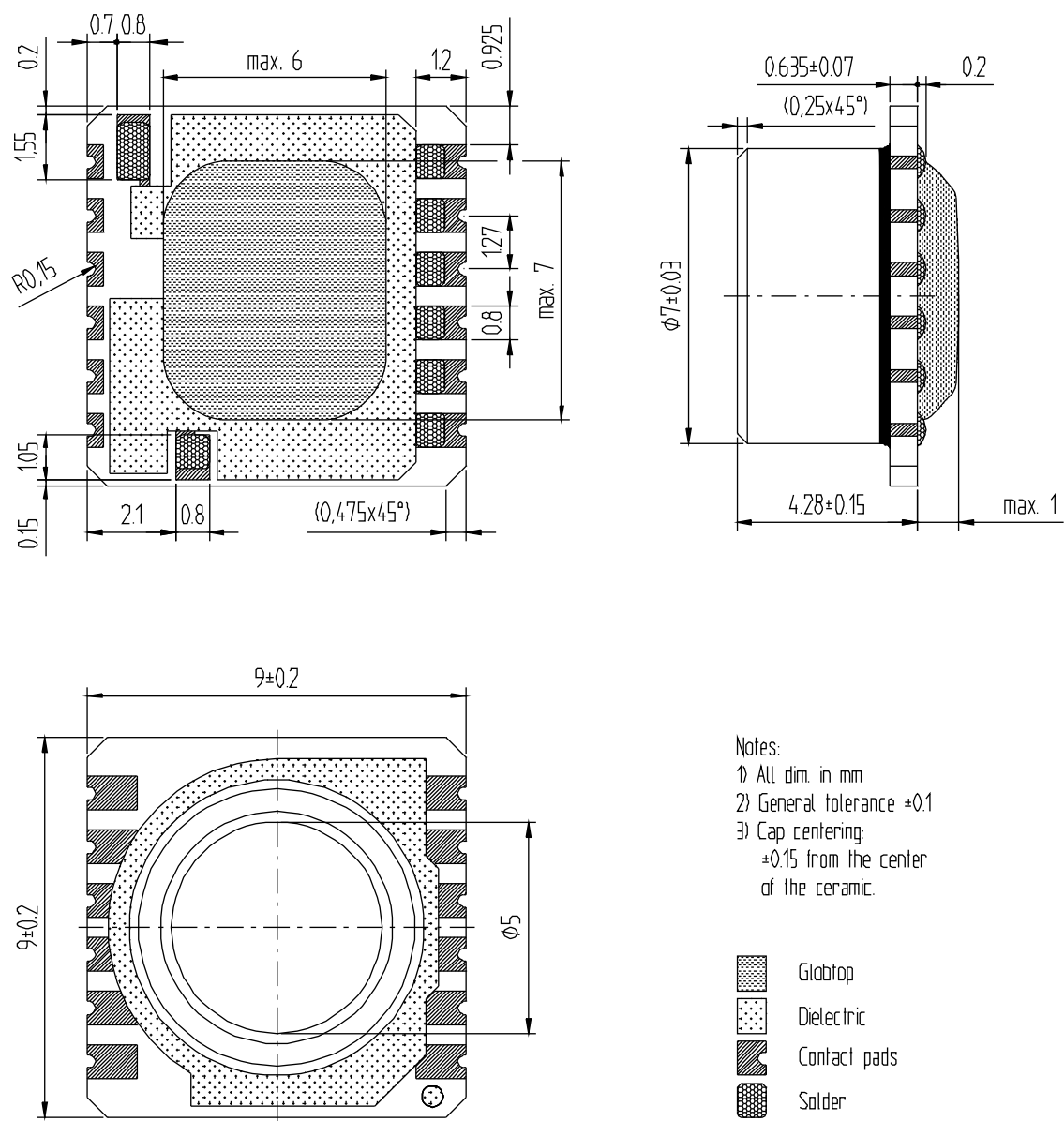
Fig. 8: Device package outlines of MS5535AM (RoHS) .
