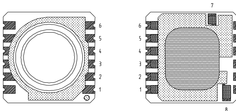
Fig. 2: Pin configuration of MS5535A (RoHS).
