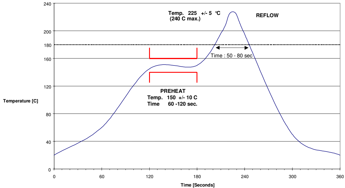
Fig. 10: Recommended soldering profile
