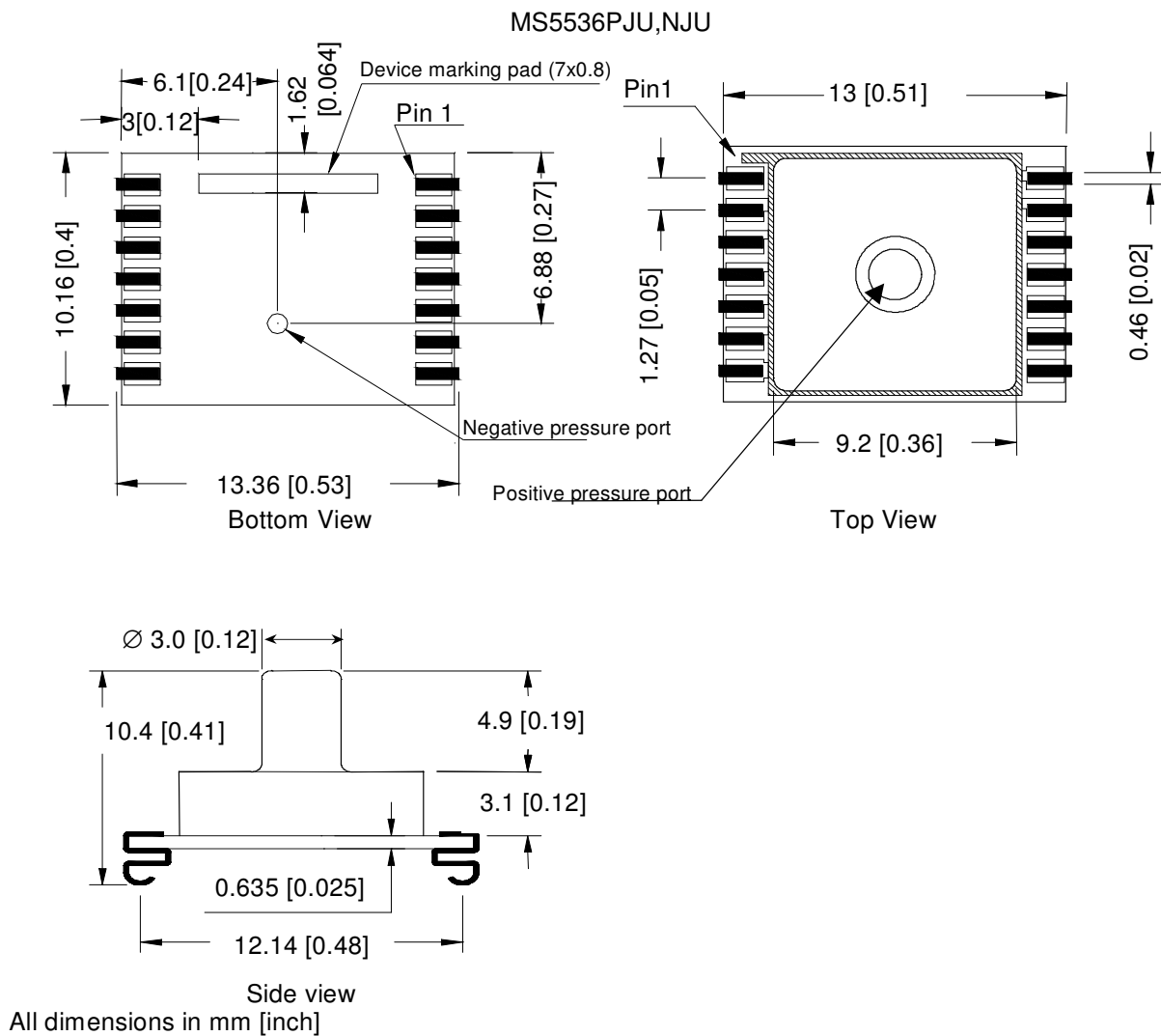
Fig. 8: Device package outlines of MS5536PJU / MS5536NJU
